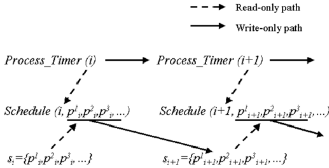
Fig. 4. Real-time algorithm.
