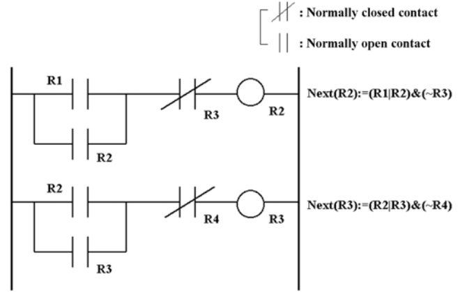
Fig. 5. Latch algorithm.
