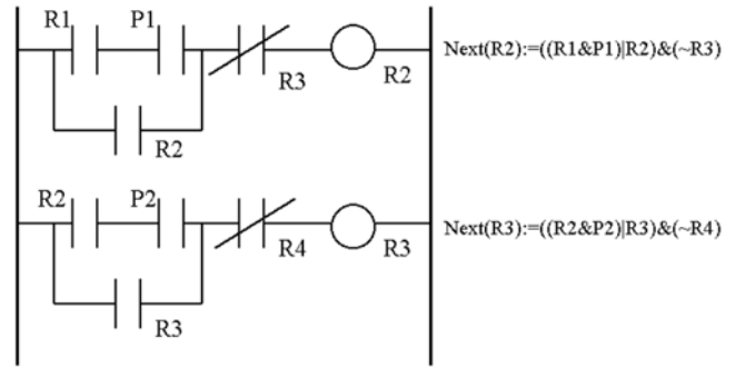
Fig. 6. Latch algorithm with precondition variables.
